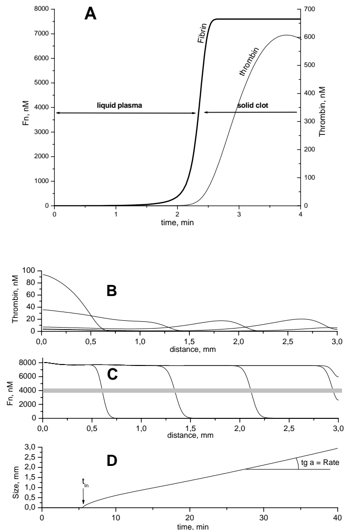
Figure 2. Simulated clotting kinetics in stirred (A) and non-stirred (B-D) normal plasma. (A): thrombin(t) and Fn(t); triggering to clotted state occur upon about 50% Fg conversion to Fn. Non-stirred system: (B) thrombin(x,t) and (C)
