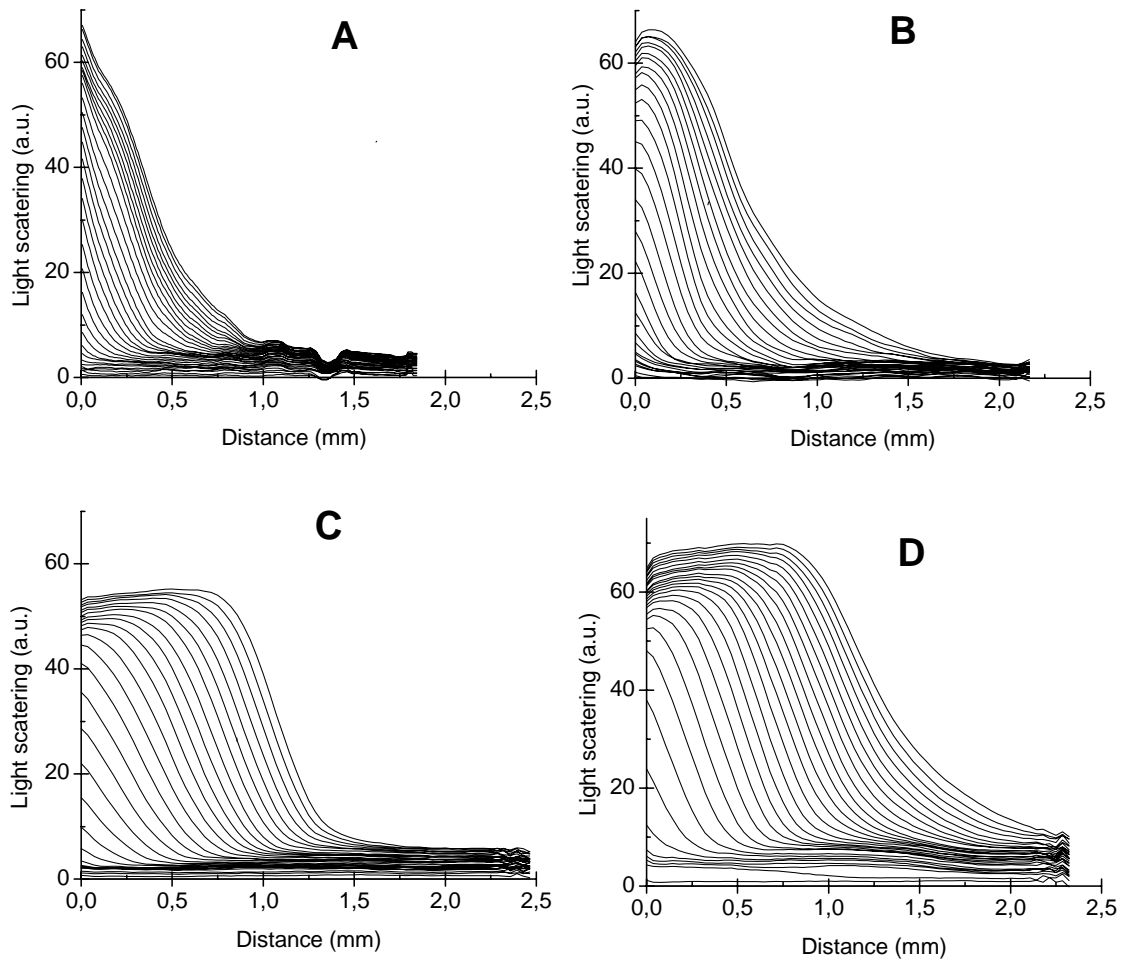
Figure 5. Clot growth from the glass surface in plasma of patients with (A) less than 1%, (B) 1.8%, (C) 2.8%, and (D) 5.5% of normal FIX clotting activity. The first curve was recorded in less than 1 minute after the start of the experiment; all other curves were recorded at a 2-minute intervals.
