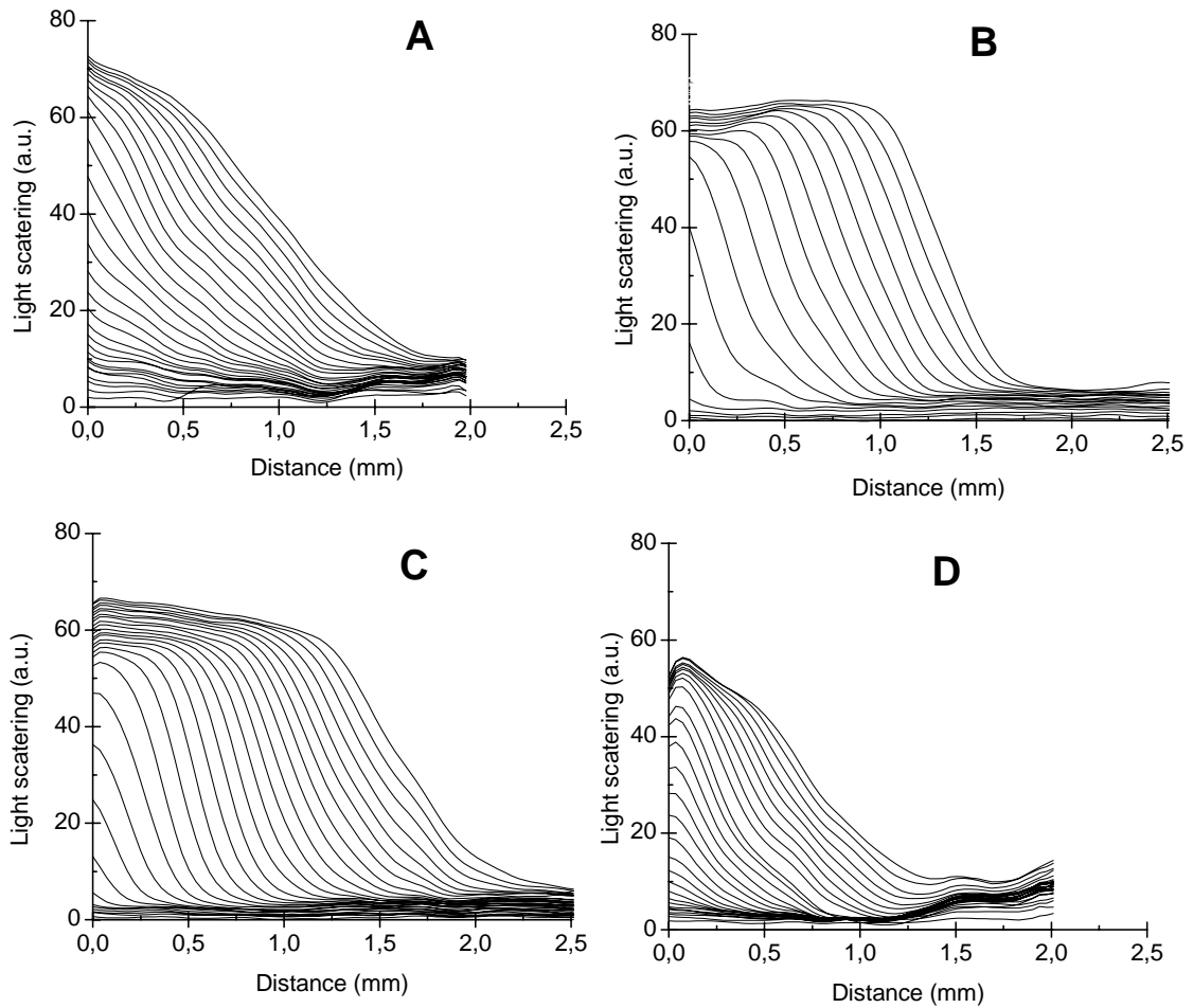
Figure 6. Clot growth in patient plasma taken (A) before and (B) 0.5, (C) 21, (D) 48 h after a single administration of Ahemphil B (200 IU/kg). On each panel, the first curve was recorded in less than 1 min after the start of the experiment; all other curves were recorded every 2 min after the first one.
