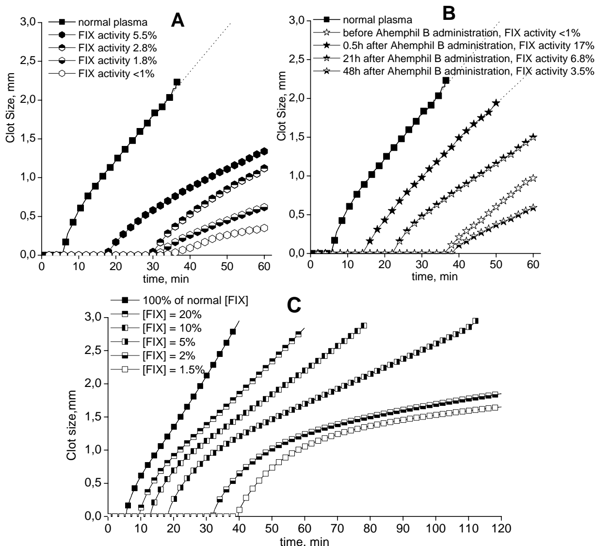
Figure 8. Influence of FIX clotting activity on clot growth kinetics in glass-activated plasma in experiment (A, B) and model (C). Note the lag-phase (clot size=0) followed by the growth phase. Experimental curves are extrapolated by the dot lines if the spontaneous clotting didn't allow to determine the clot size at t=60 min.
