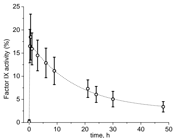
Figure 7. FIX clotting activity (percentage of the norm) before and after the single dose (200 IU/kg) of FIX concentrate Ahemphil B administration. The data are means for five patients with the basal FIX level less than 1%. Their FIX level increased to 18.5 \pm 5\% in 30 min after administration and then exponentially decreased ( t_{1/2} = 12\text{h} ) to 3.5 \pm 1.1\% over the subsequent 48 h.
