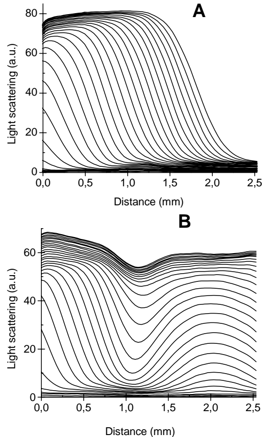
Figure 4. Clot grows away from the glass surface in a healthy donor plasma. Curves are light scattering profiles at 2-minutes time intervals. A: no spontaneous foci of activation on the way of the clot; B: interaction with a clot spontaneously formed at a 2-mm distance from the activator.
