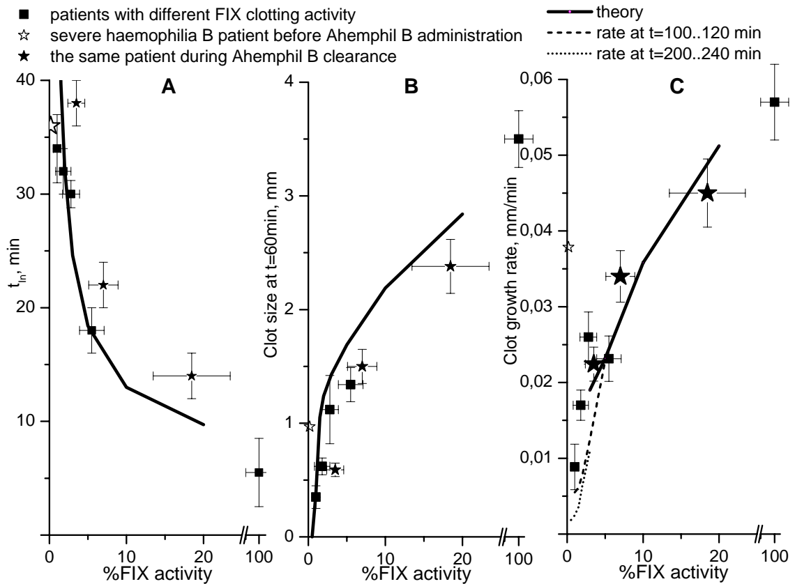
Figure 9. Parameters of clot growth kinetics in experiment (points) and model (lines): (A) time of clot growth initiation t_{in} , (B) clot size at t=60 min, (C) activator-distanced rate of clot growth. For experiment, error bars are shown. Solid, dashed and dotted lines show rate calculated further and further from the activator: at time intervals 50..60, 100..120 and 200..240 min, respectively. Combined these lines show the steady clot growth rate in the model.
