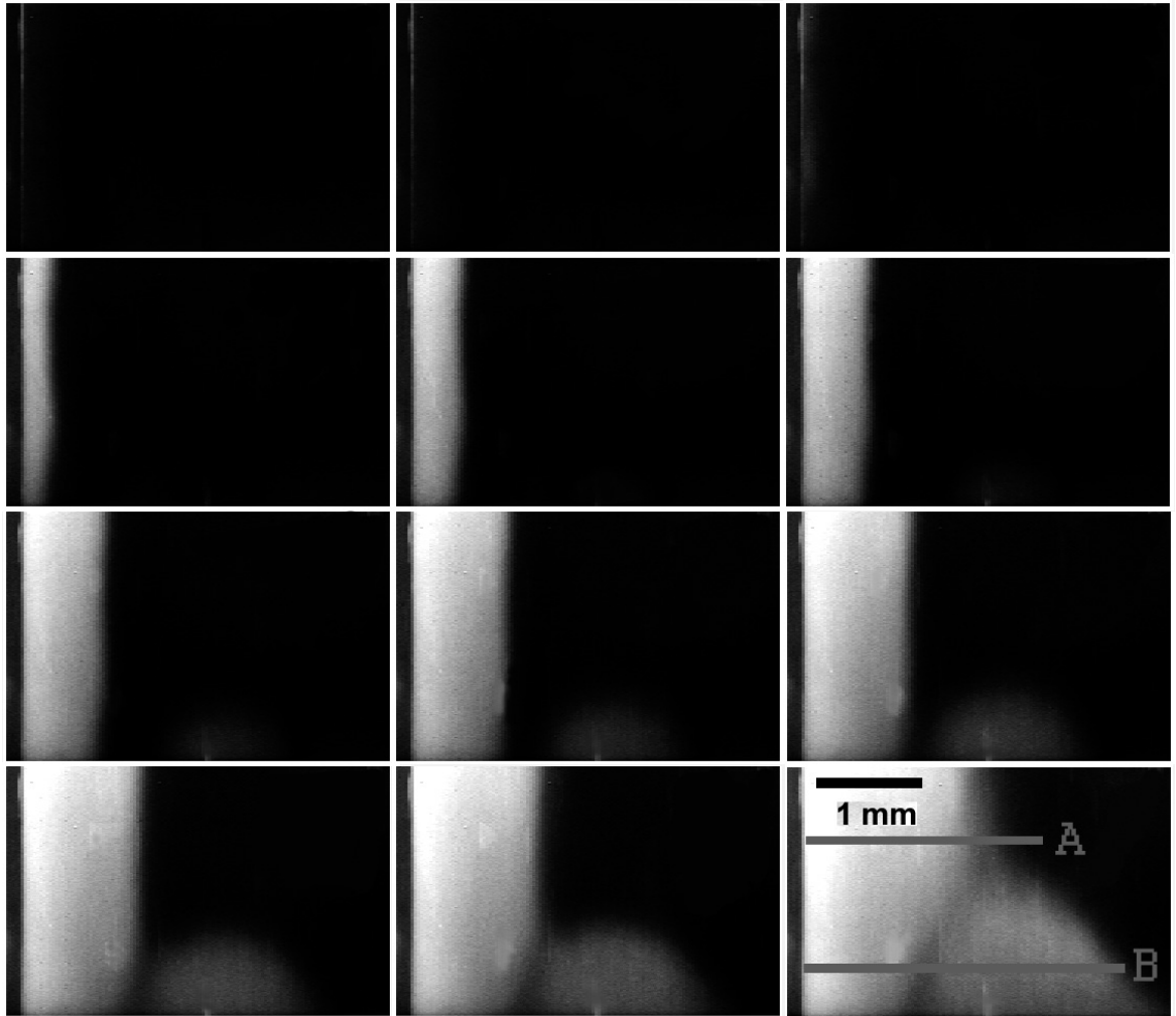
Figure 3. Spatial dynamics of clot growth in healthy donor plasma activated by contact with the glass surface (leftmost vertical line in each frame). In images, clot is light, and liquid plasma is dark. The first frame was taken 2 min after the recalcification, the subsequent at 4 min intervals. The last frame corresponds to 46 min after recalcification. The light scattering intensity profiles on fig.4 A and B were obtained along the straight lines indicated on the last frame.
